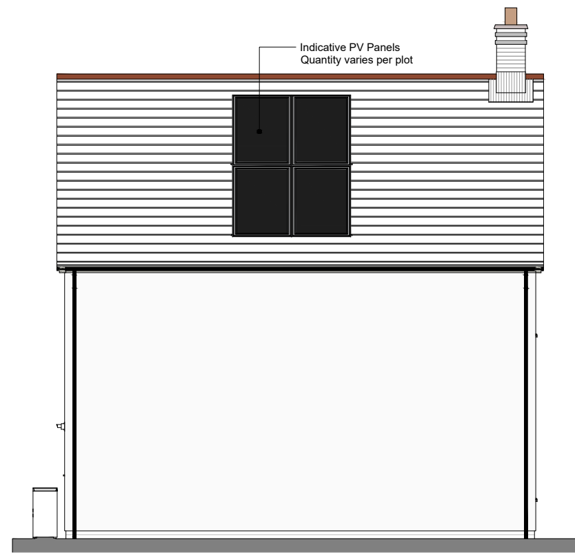
Side Elevation
