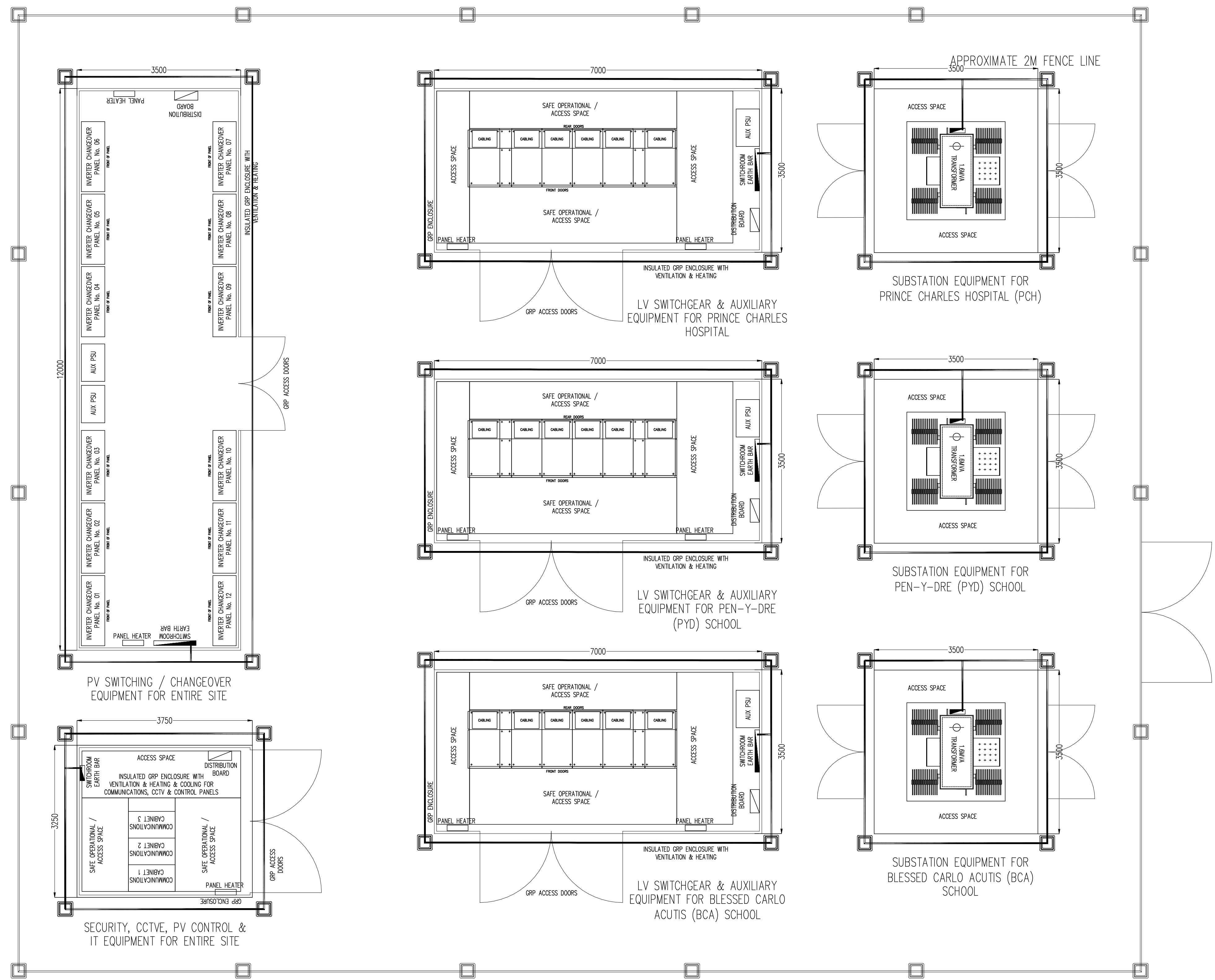
PV Compound Details 1:50
