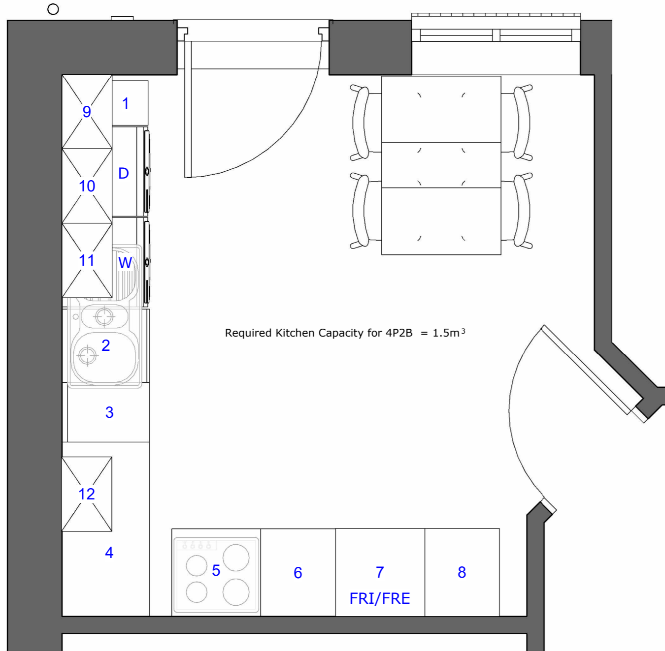
1 Kitchen Layout - 4P2B House 1 : 25
