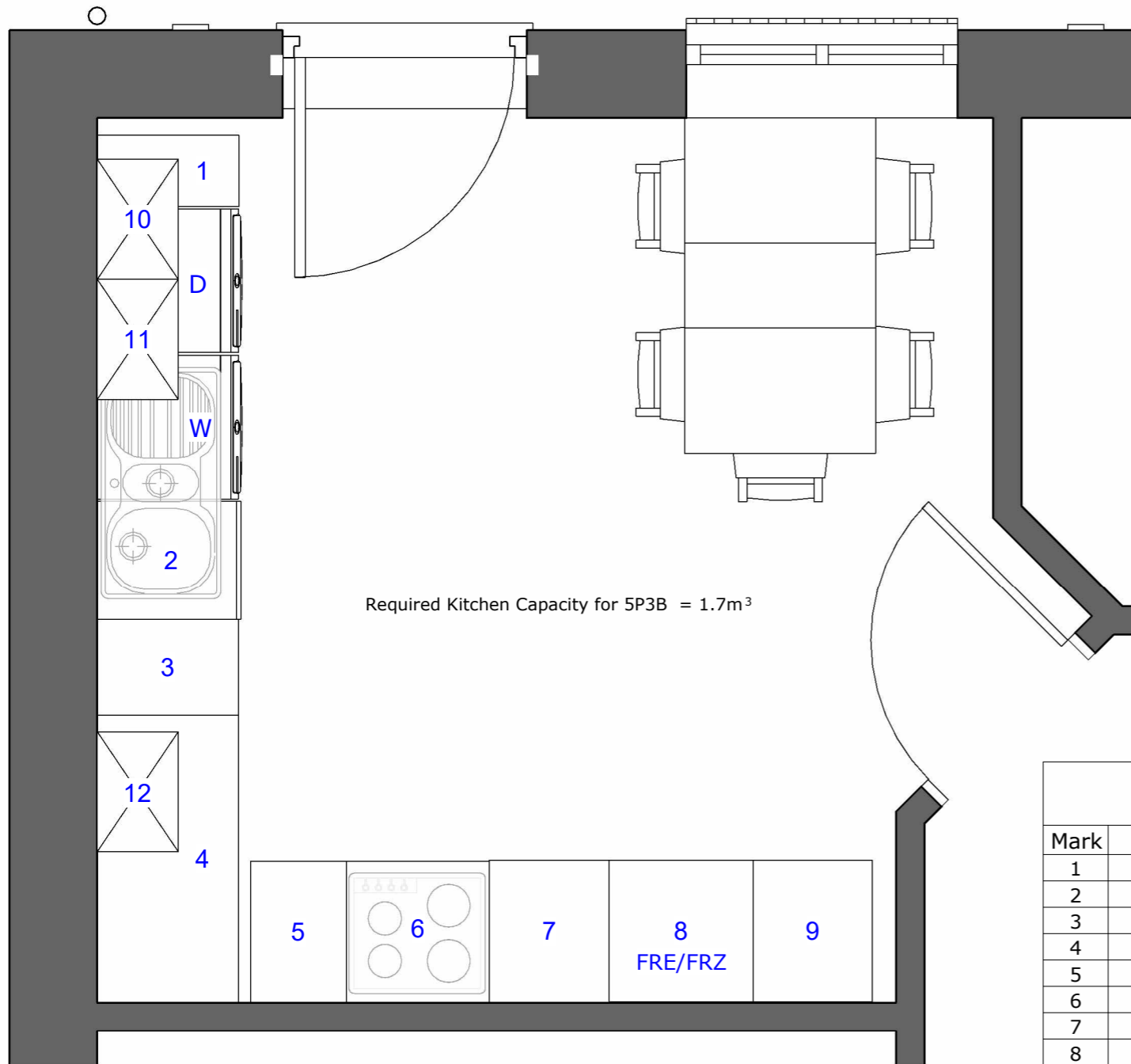
1 Kitchen Layout - 5P3B House 1 : 25
