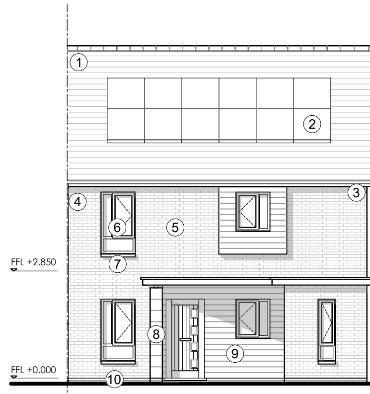
FRONT ELEVATION
