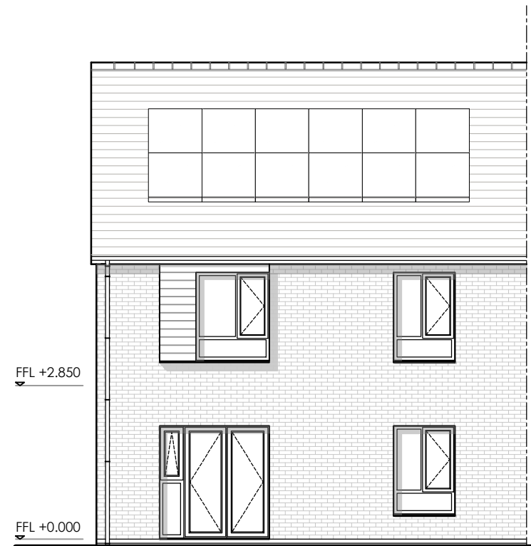
REAR ELEVATION
