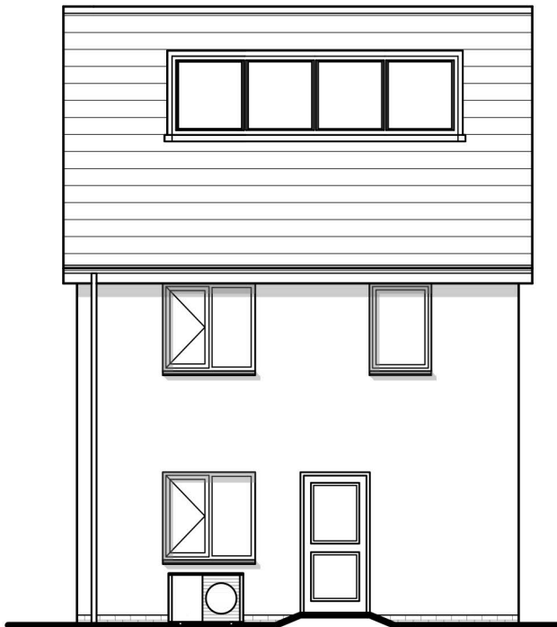
REAR ELEVATION
