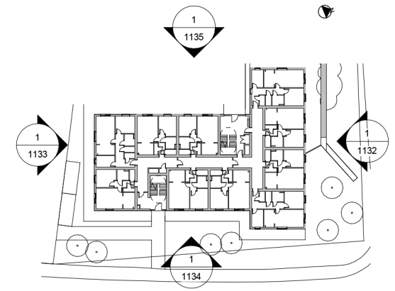
Key Plan 1:500
